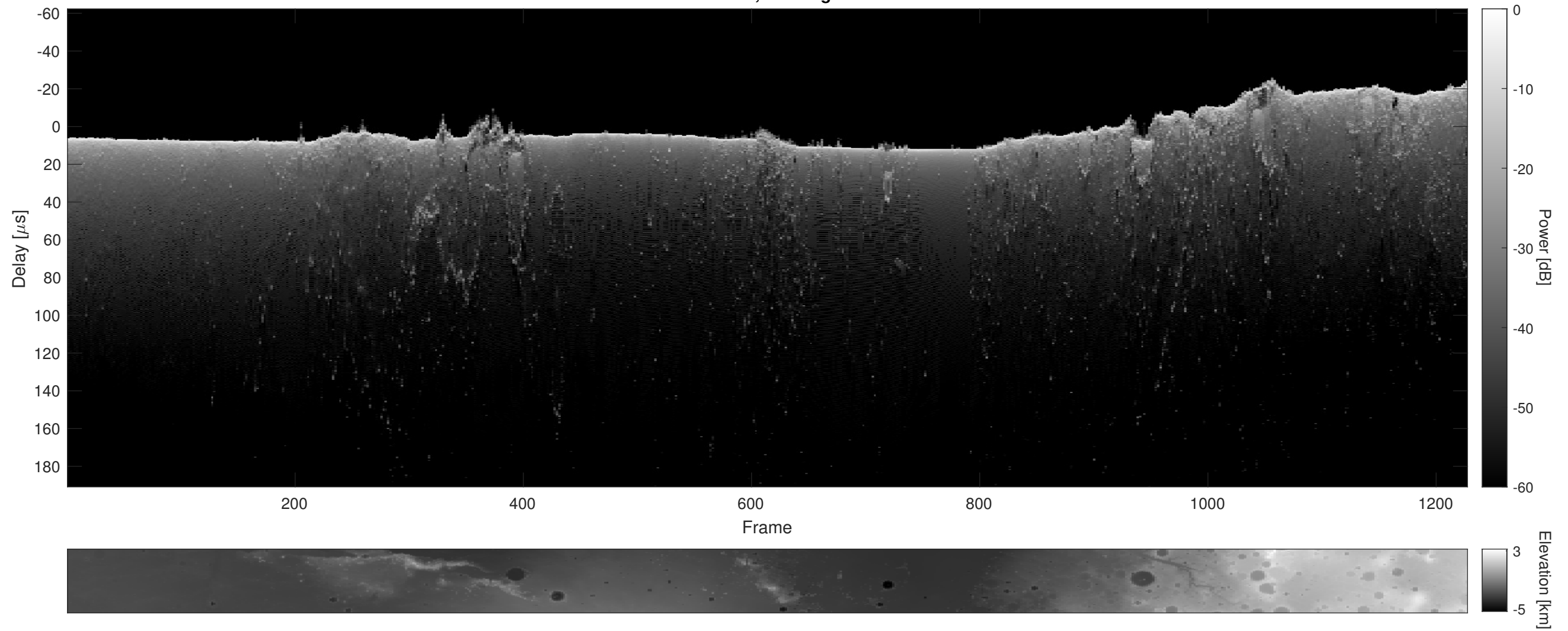
Orbit 5190, Cluttergram
