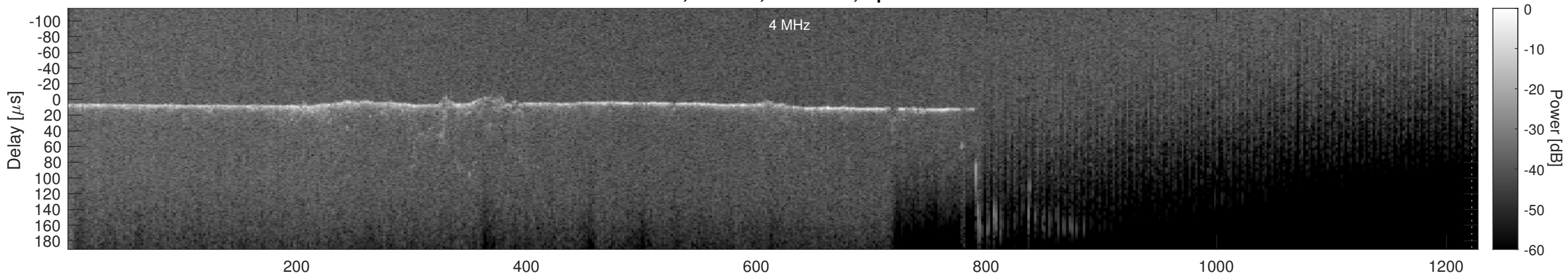
Orbit 5190, Cluttergram
