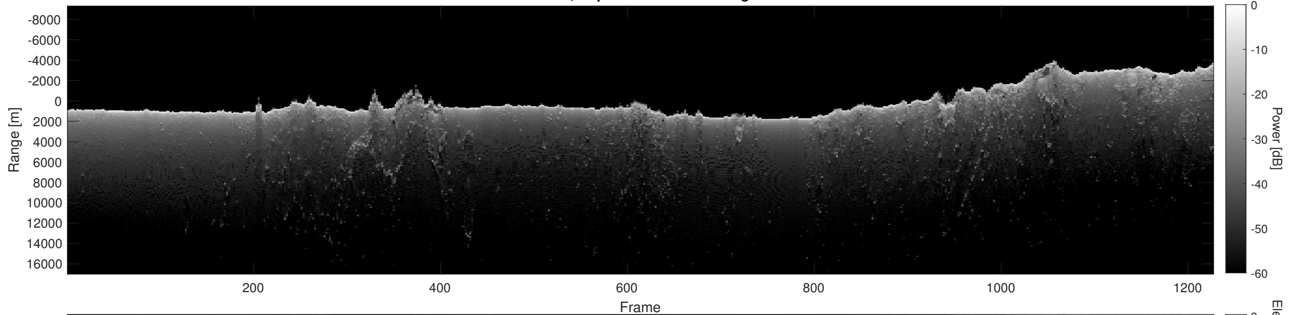
Orbit 5190, Depth-Corrected Cluttergram
