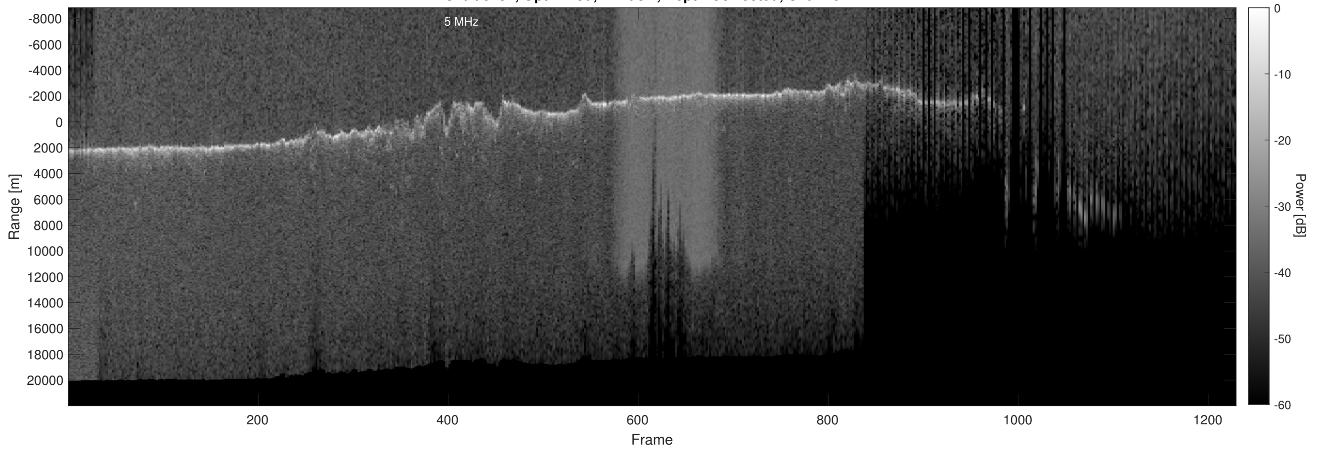
Orbit 5191, Optimized, Window, Depth-Corrected, Channel 2
