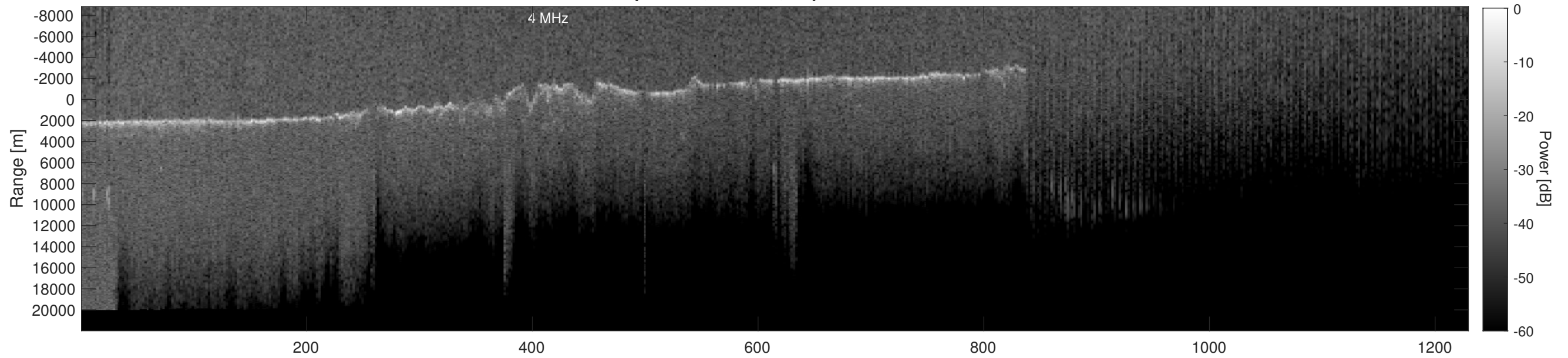
Orbit 5191, Depth-Corrected Cluttergram
