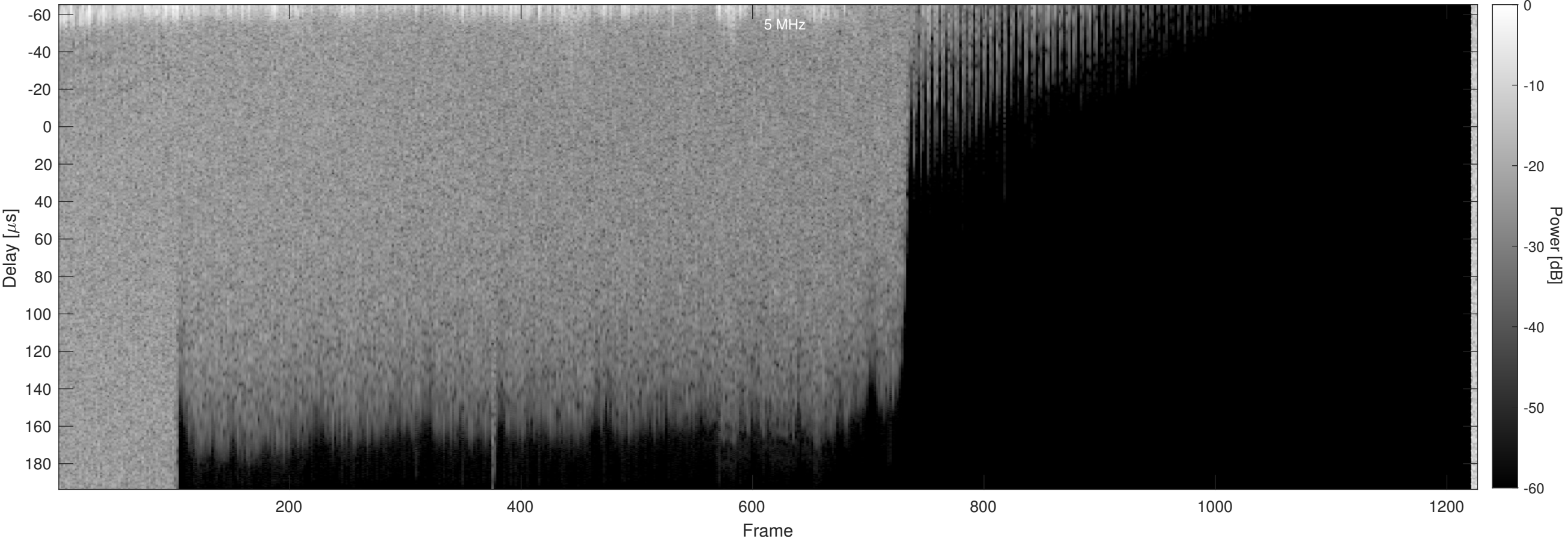
Orbit 5192, Chapman, Window, Channel 2
