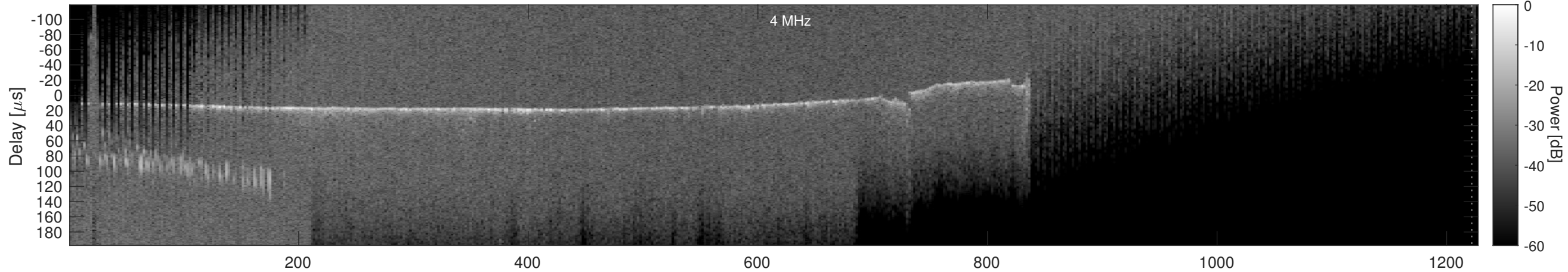
Orbit 5194, Cluttergram
