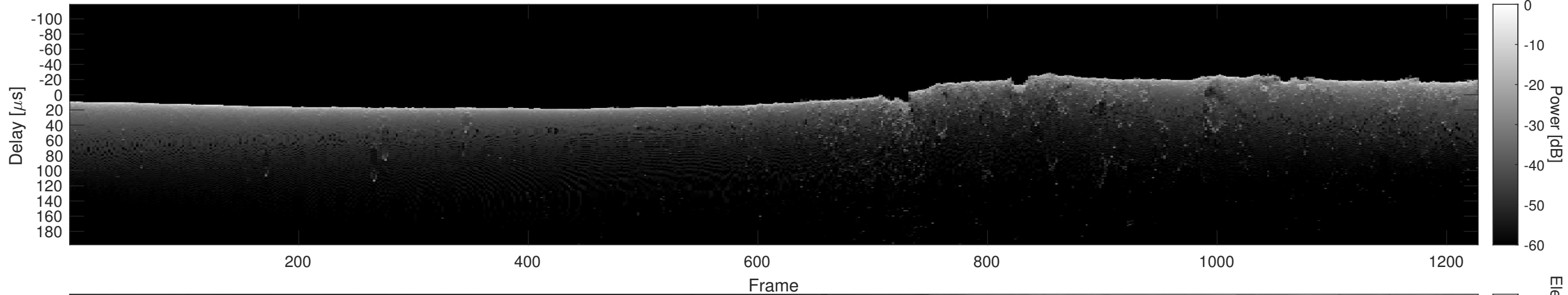
Orbit 5194, Cluttergram
