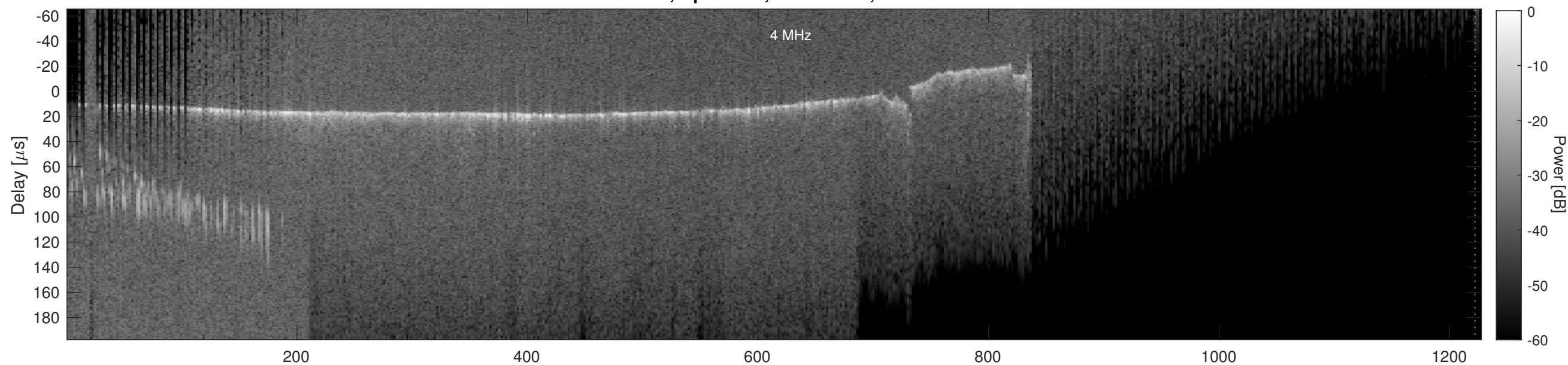
Orbit 5194, Cluttergram
