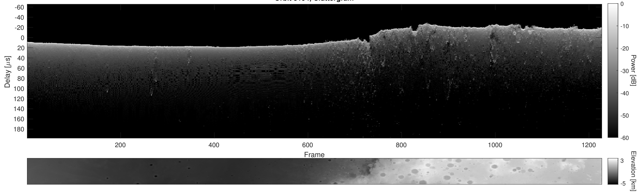
Orbit 5194, Cluttergram
