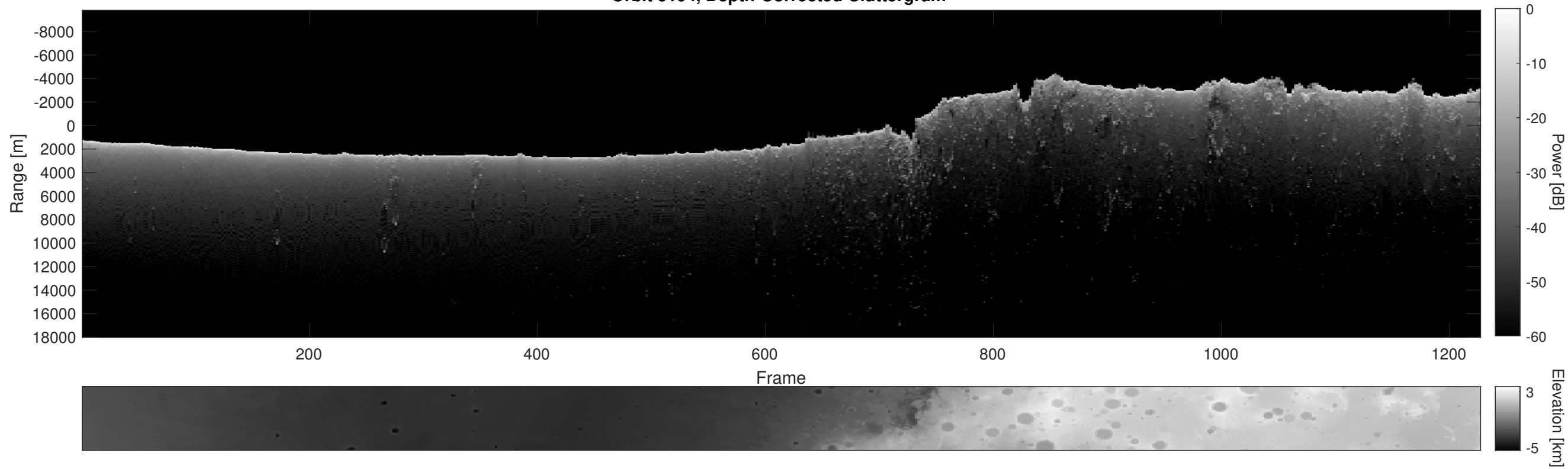
Orbit 5194, Depth-Corrected Cluttergram
