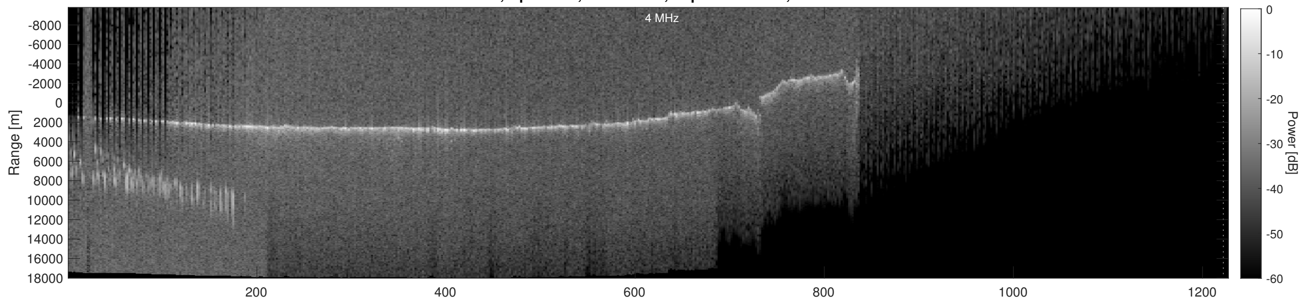
Orbit 5194, Depth-Corrected Cluttergram
