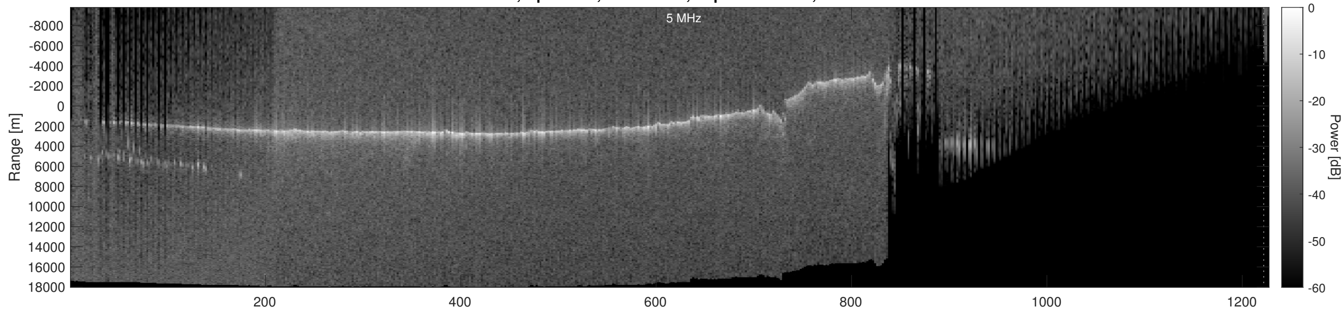
Orbit 5194, Optimized, No Window, Depth-Corrected, Channel 2
