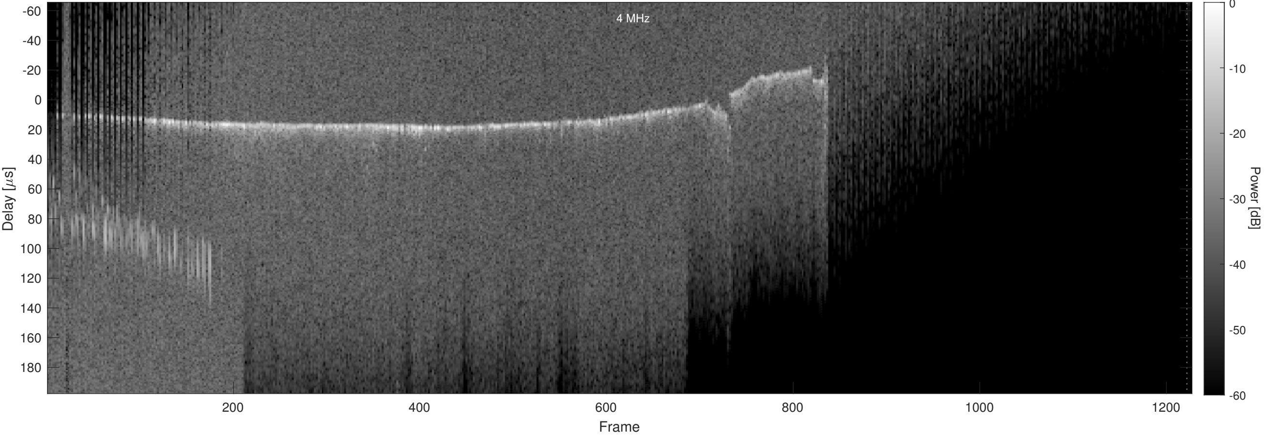
Orbit 5194, Optimized, Window, Channel 2
