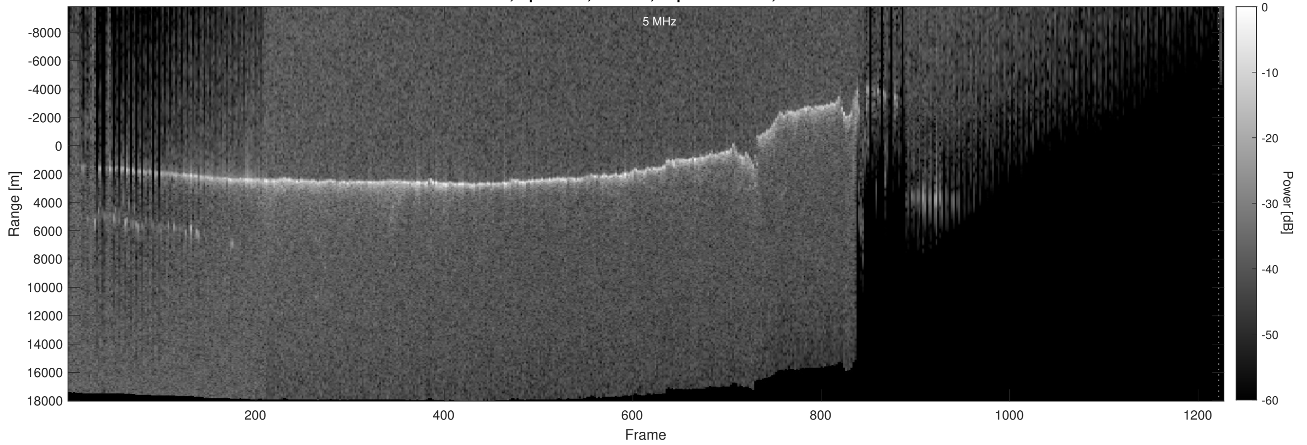
Orbit 5194, Optimized, Window, Depth-Corrected, Channel 2
