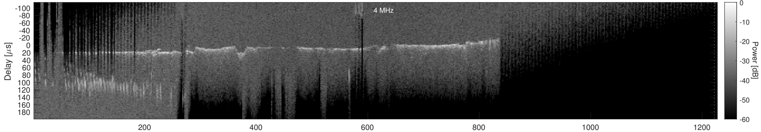
Orbit 5195, Cluttergram
