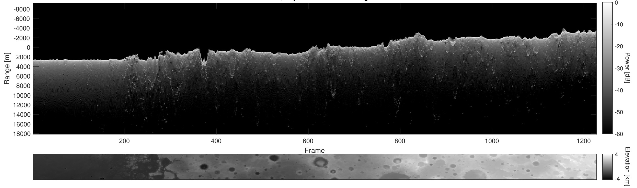
Orbit 5195, Depth-Corrected Cluttergram
