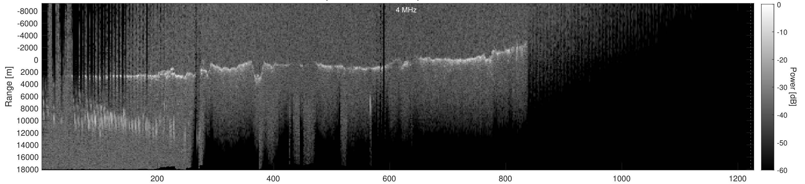
Orbit 5195, Depth-Corrected Cluttergram
