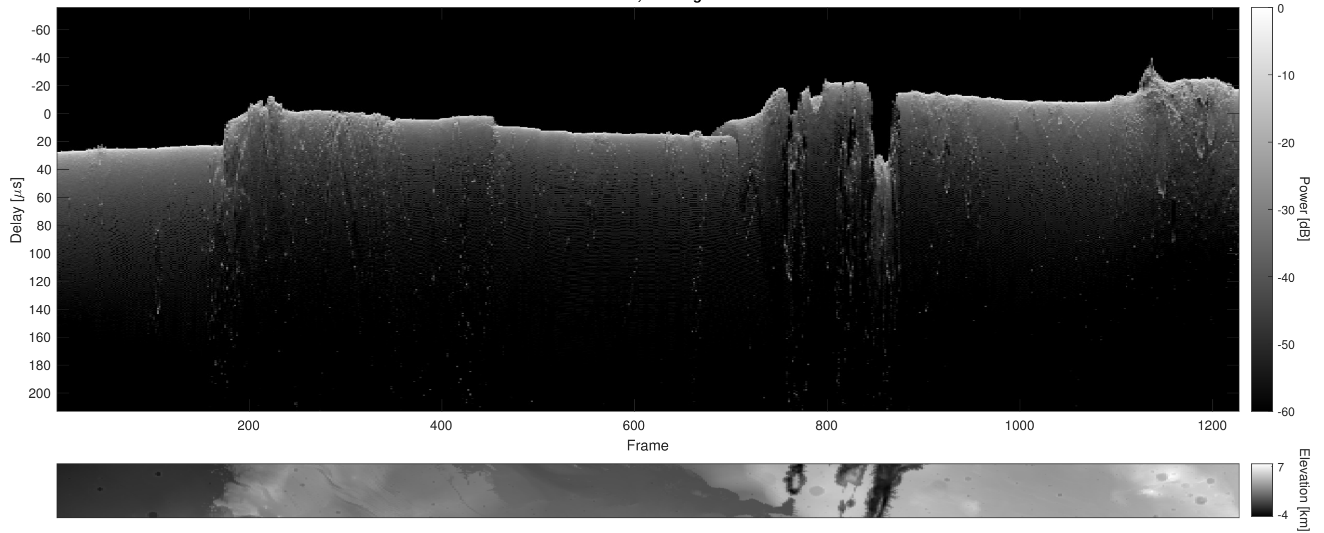
Orbit 5196, Cluttergram
