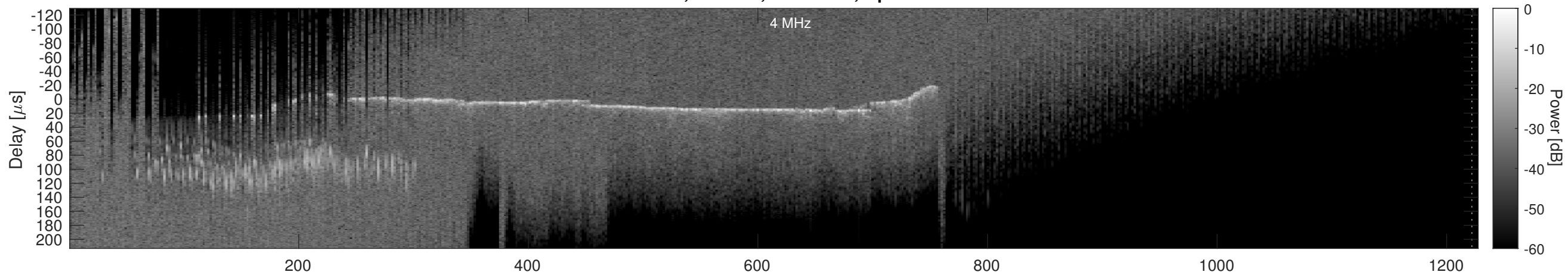
Orbit 5196, Cluttergram
