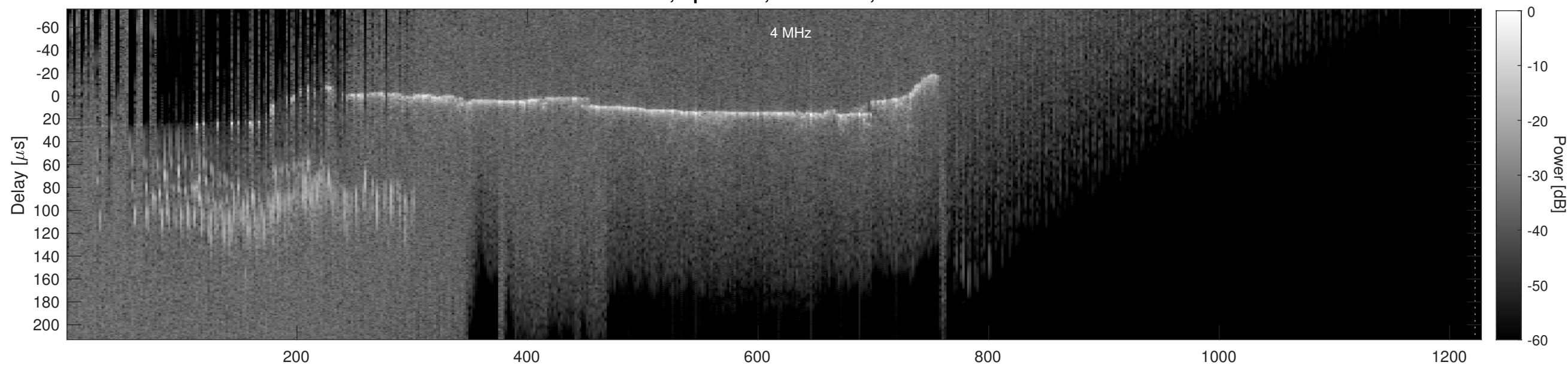
Orbit 5196, Cluttergram
