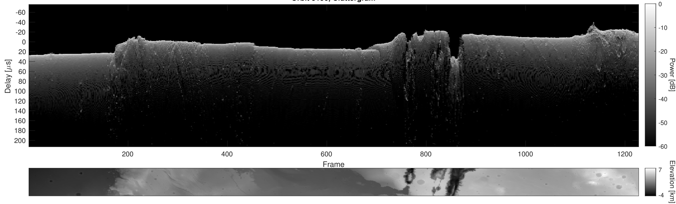
Orbit 5196, Cluttergram
