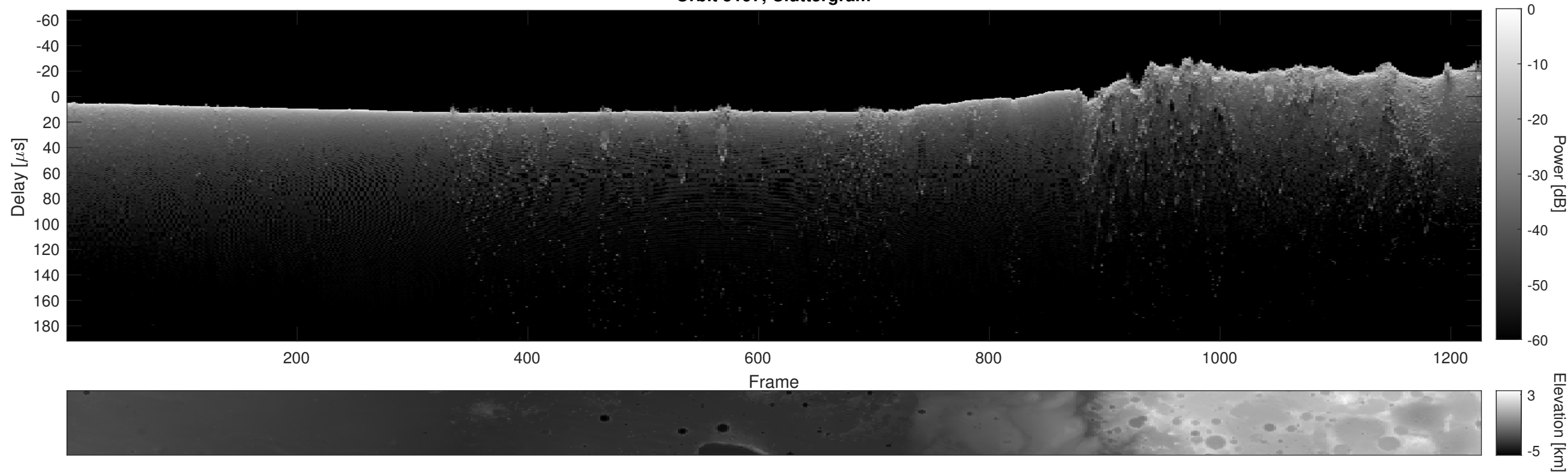
Orbit 5197, Cluttergram
