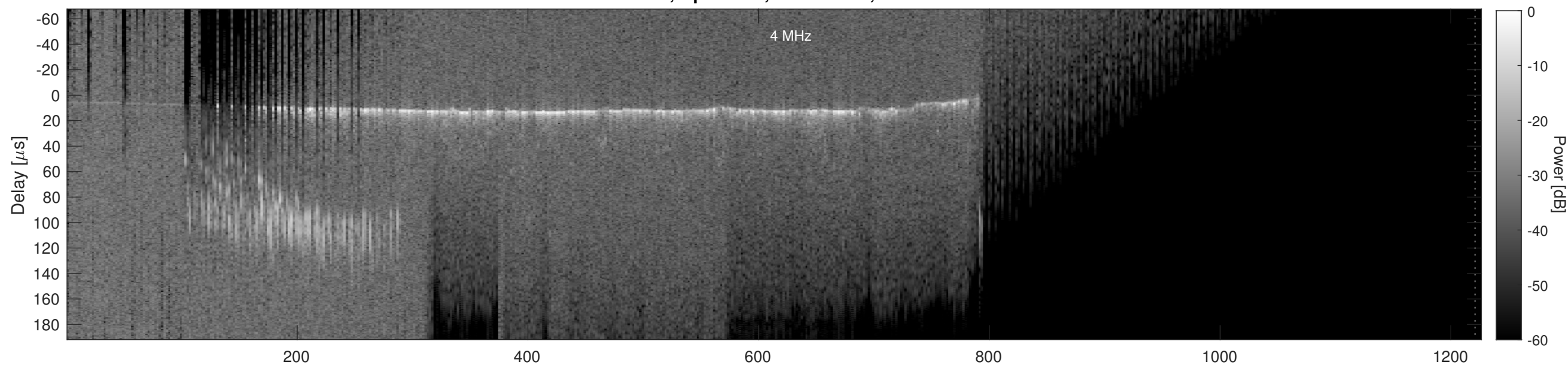
Orbit 5197, Cluttergram
