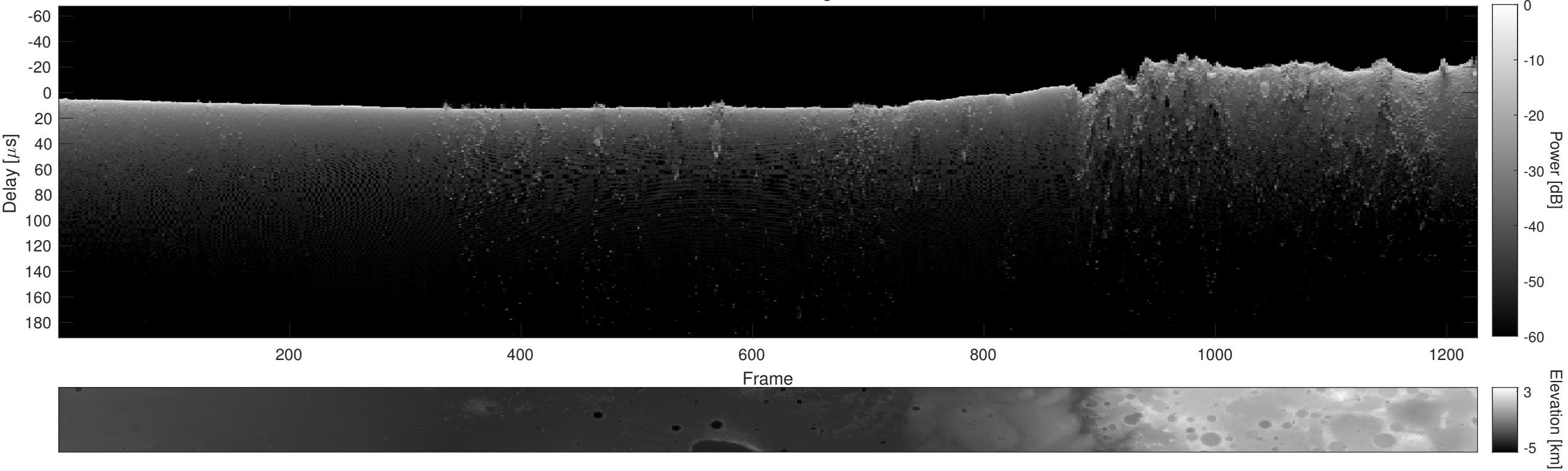
Orbit 5197, Cluttergram
