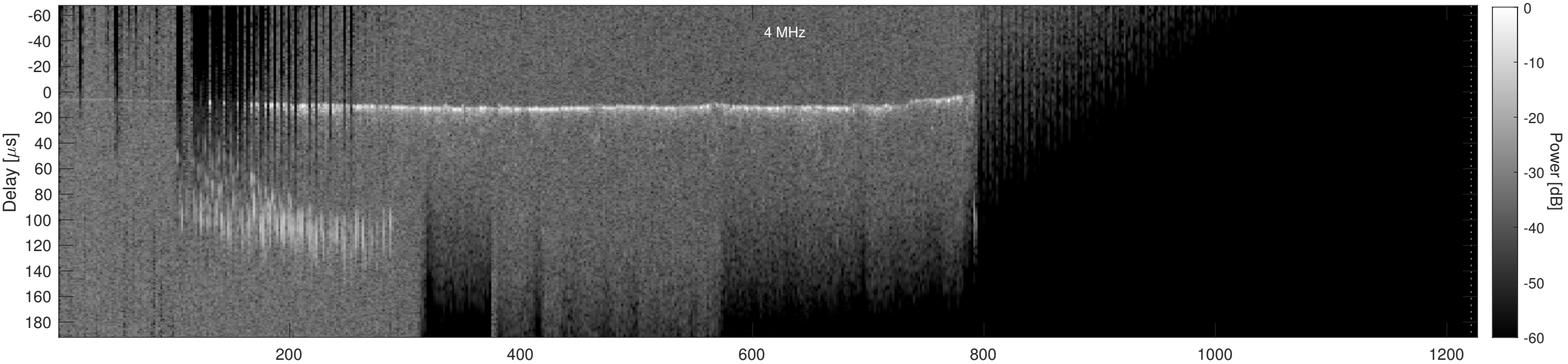
Orbit 5197, Cluttergram
