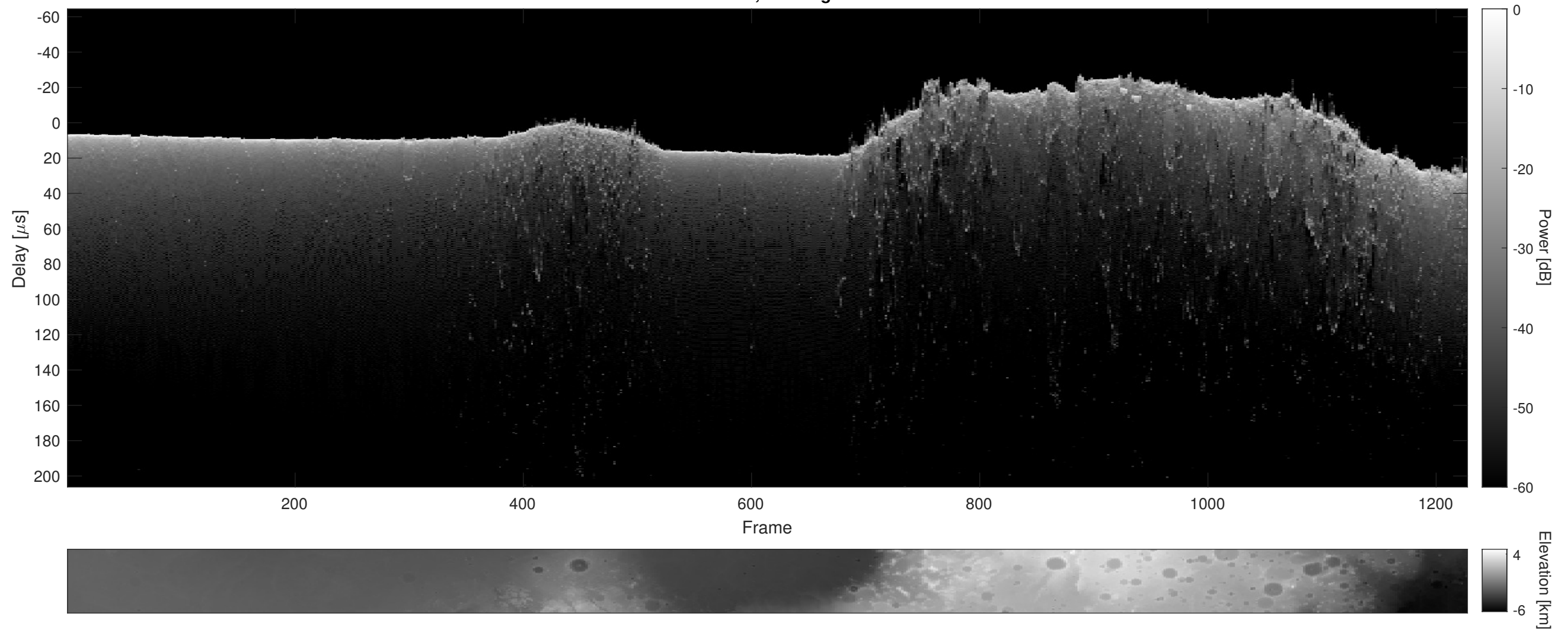
Orbit 5198, Cluttergram
