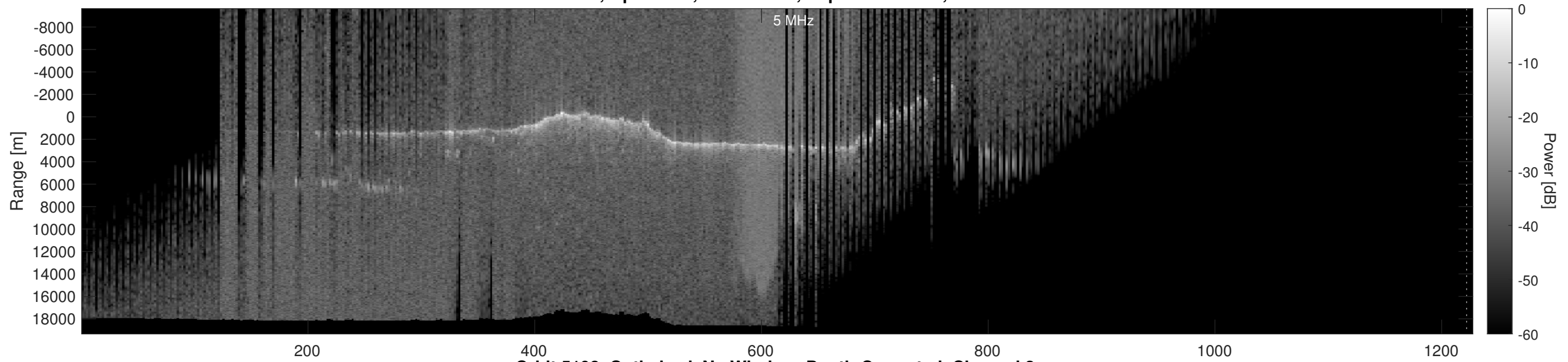
Orbit 5198, Optimized, No Window, Depth-Corrected, Channel 2
