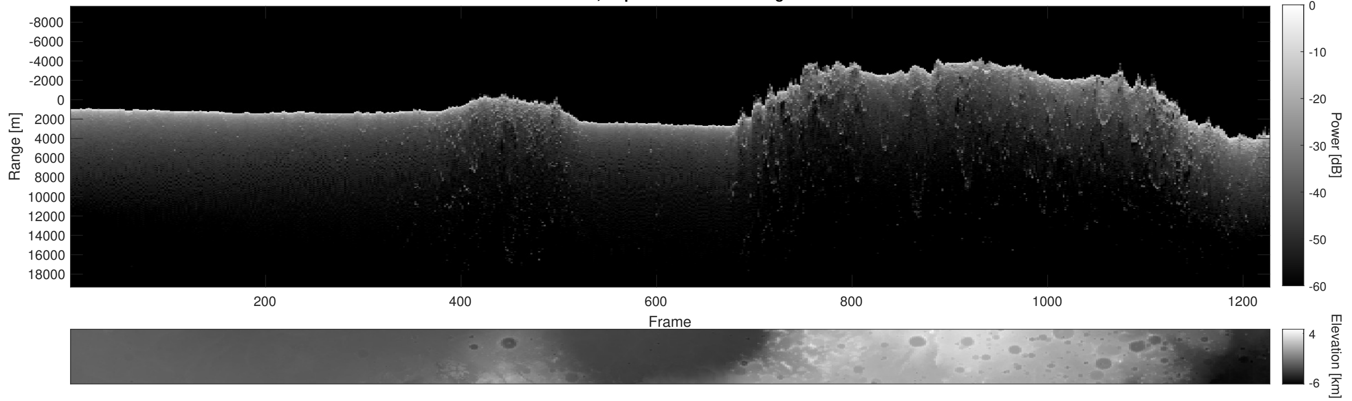
Orbit 5198, Depth-Corrected Cluttergram
