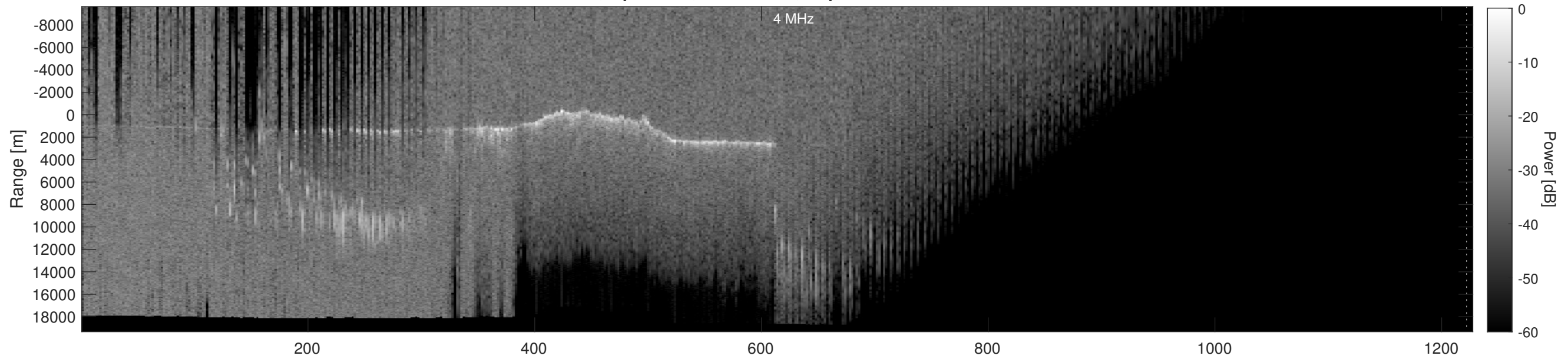
Orbit 5198, Depth-Corrected Cluttergram
