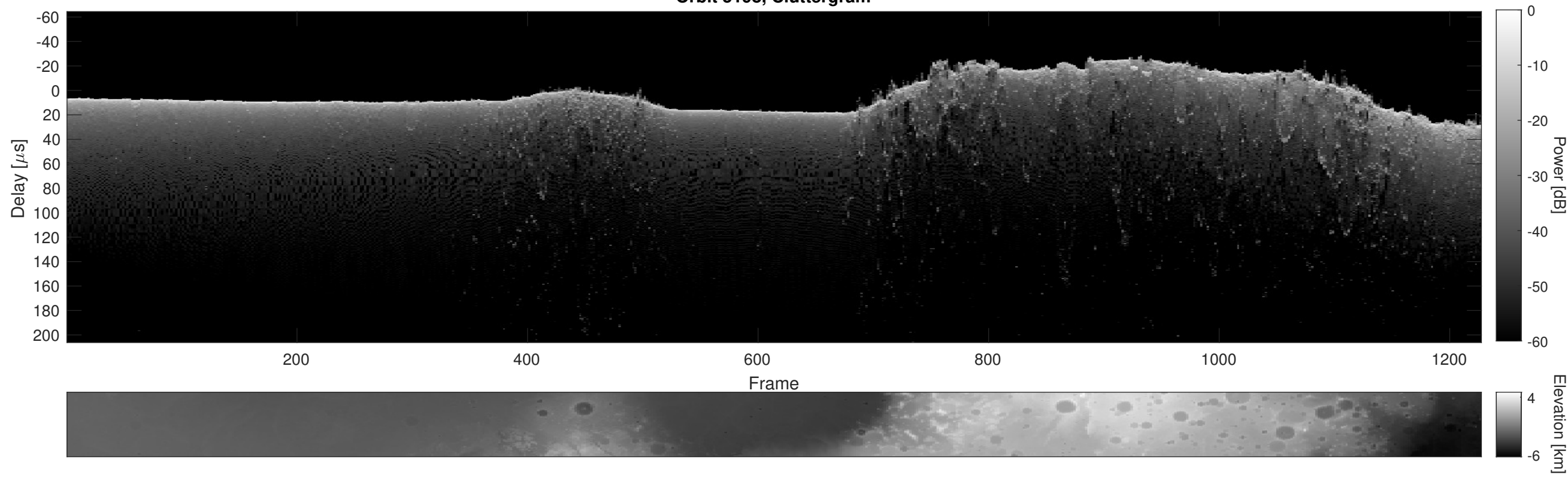
Orbit 5198, Cluttergram
