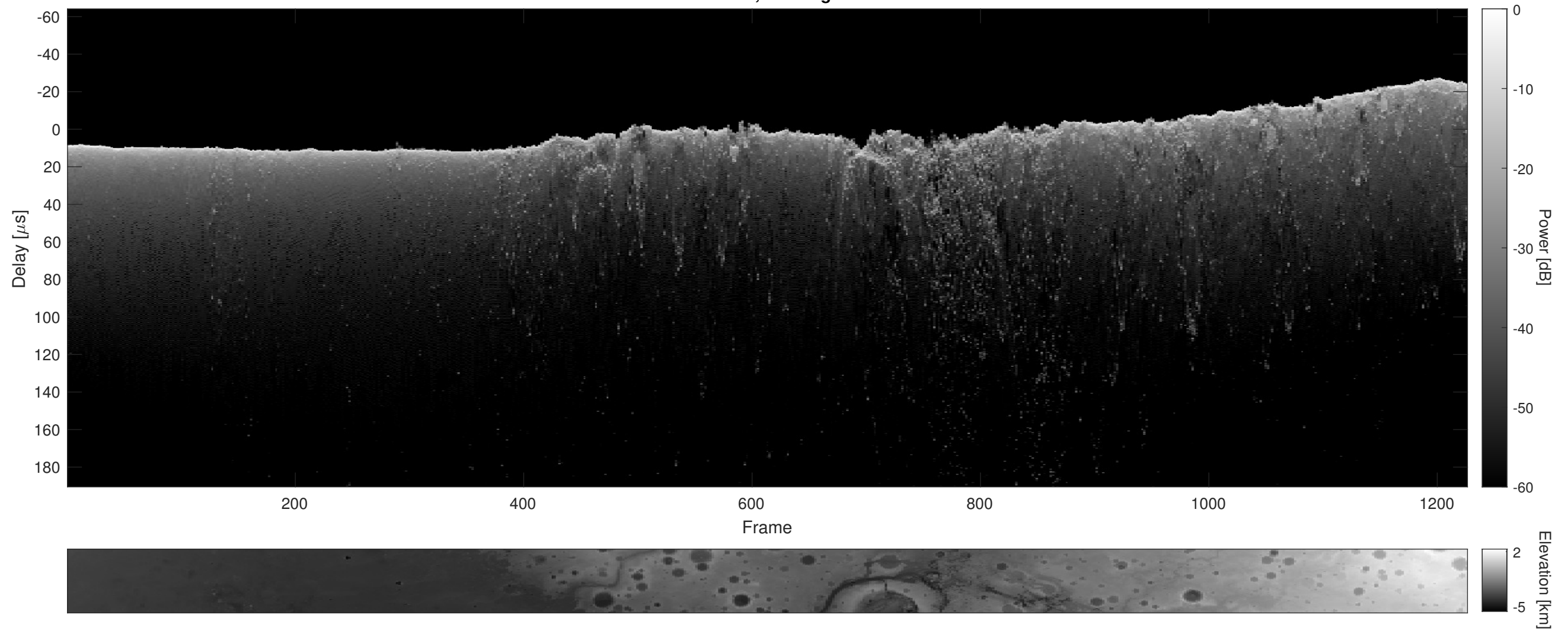
Orbit 5199, Cluttergram
