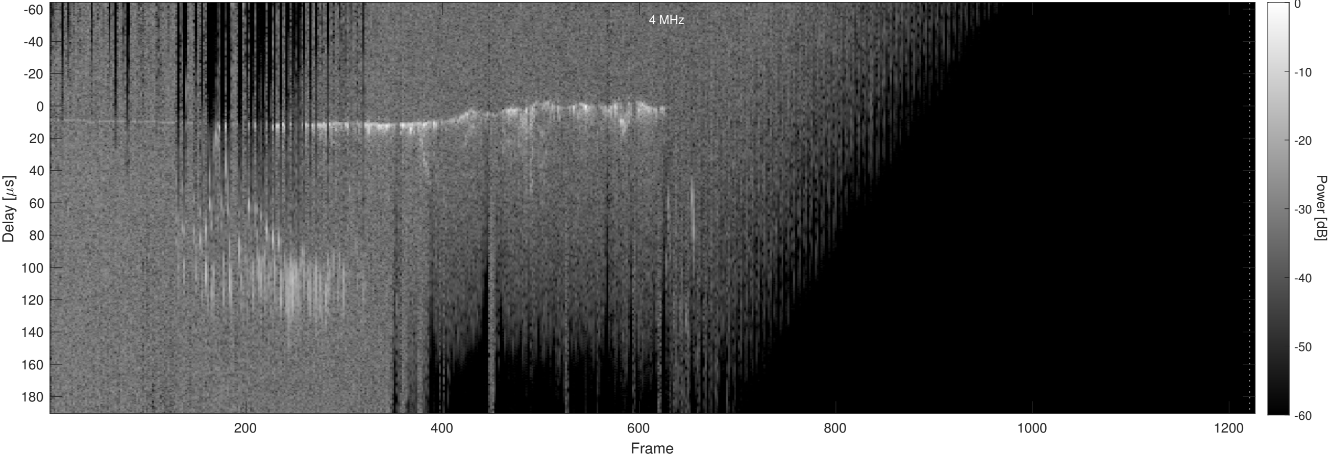
Orbit 5199, Optimized, No Window, Channel 2
