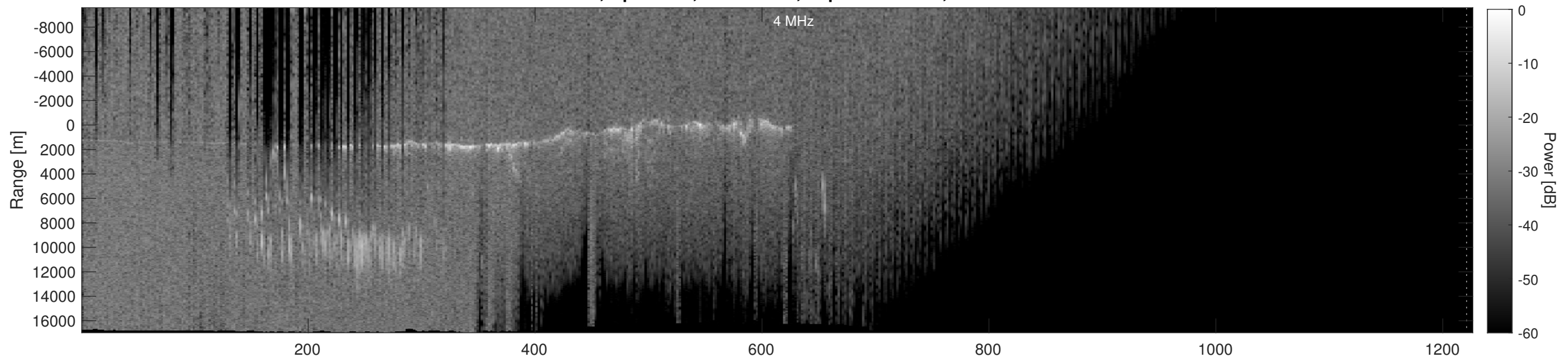
Orbit 5199, Depth-Corrected Cluttergram
