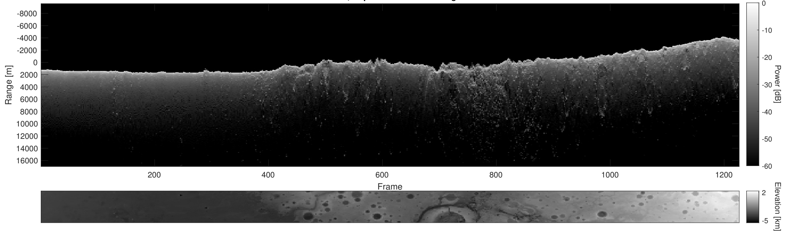
Orbit 5199, Depth-Corrected Cluttergram
