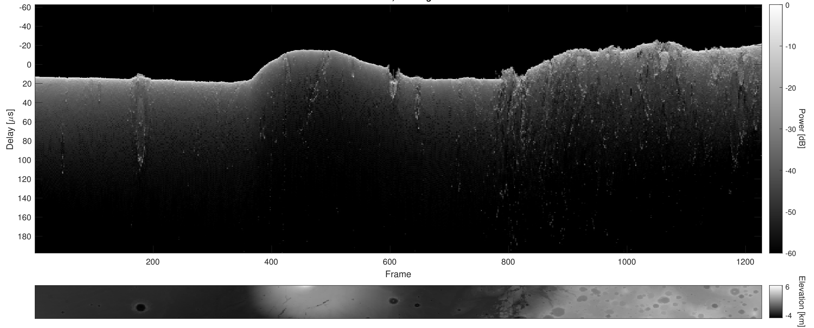
Orbit 5201, Cluttergram
