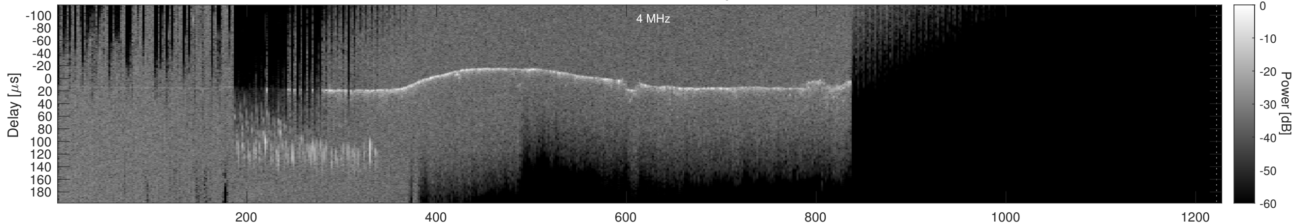
Orbit 5201, Cluttergram
