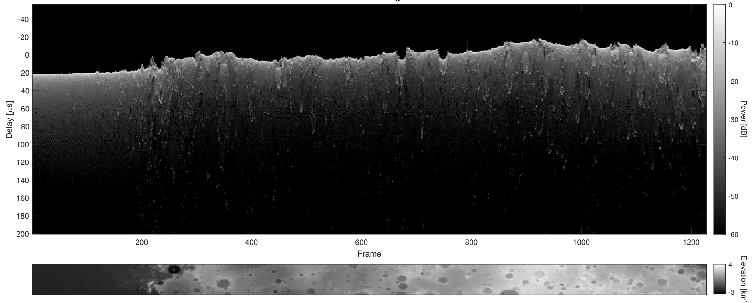
Orbit 5202, Cluttergram
