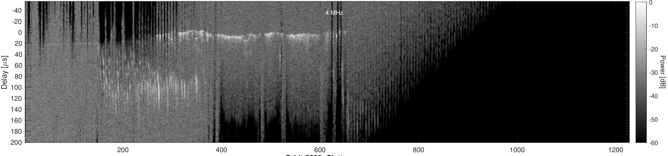
Orbit 5202, Cluttergram
