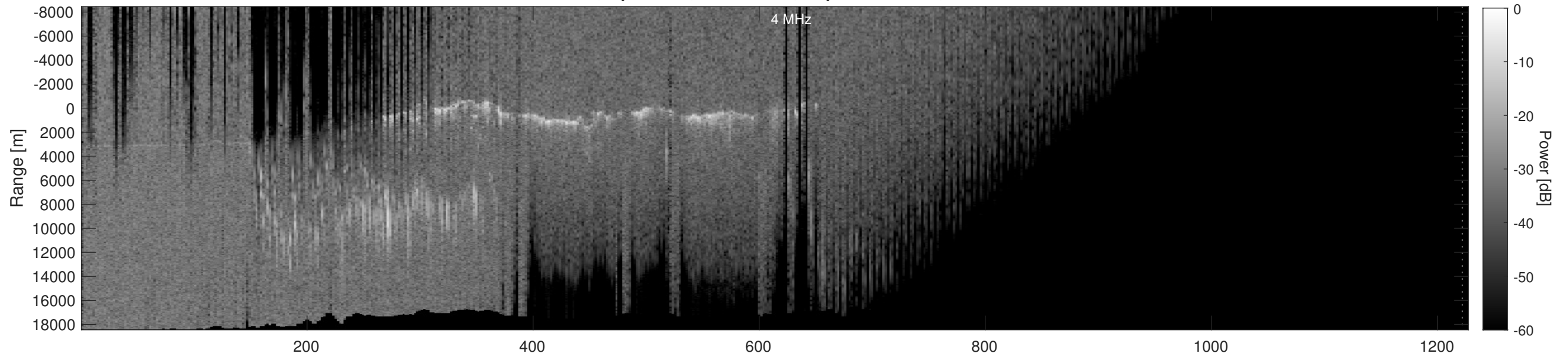
Orbit 5202, Depth-Corrected Cluttergram
