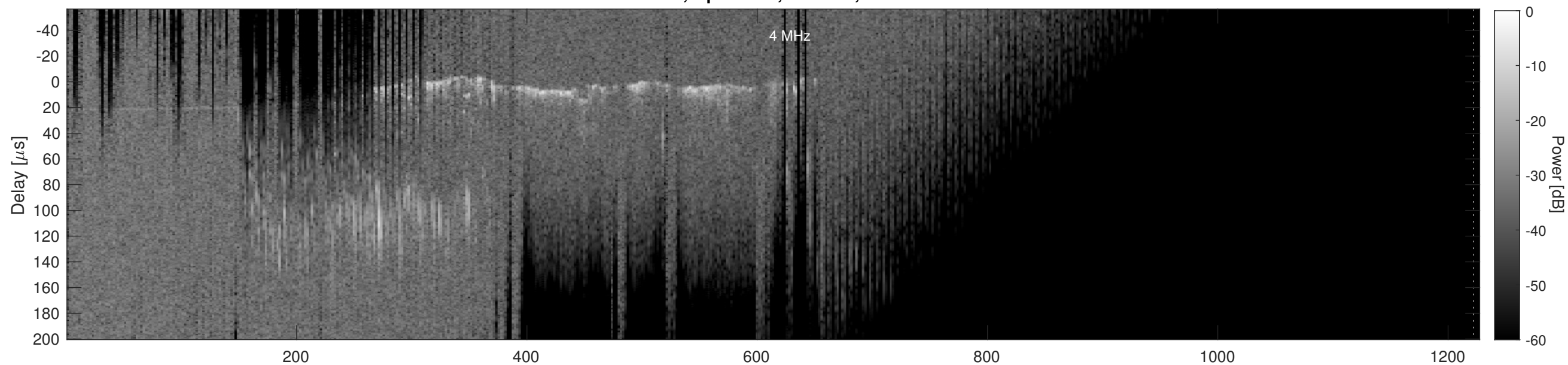
Orbit 5202, Cluttergram
