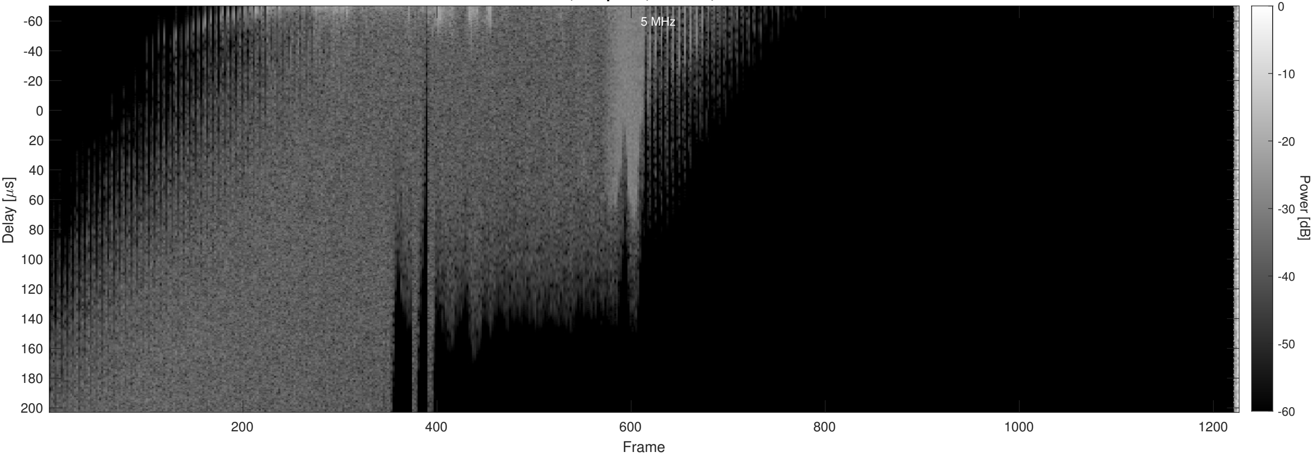
Orbit 5203, Chapman, Window, Channel 2
