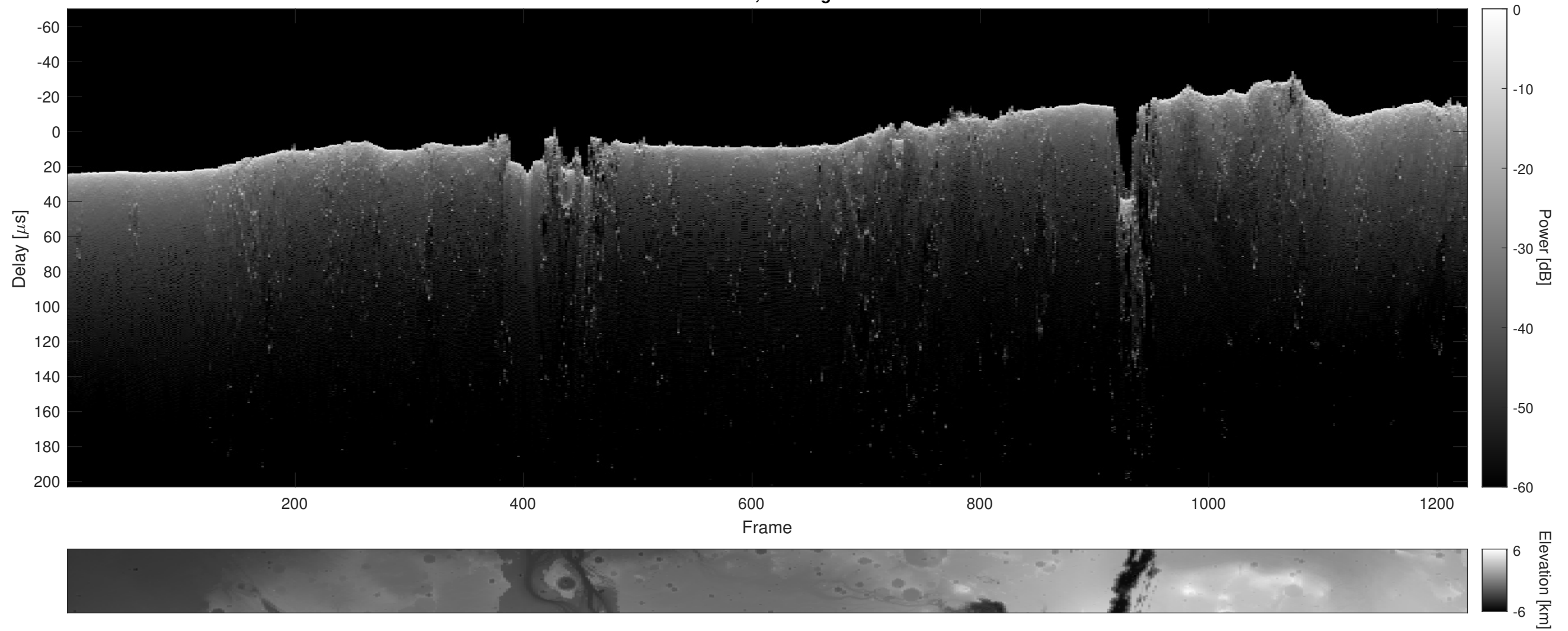
Orbit 5203, Cluttergram
