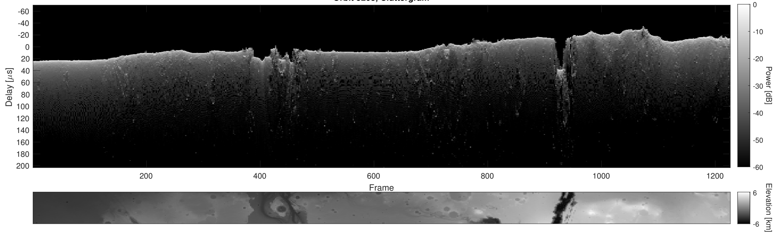
Orbit 5203, Cluttergram
