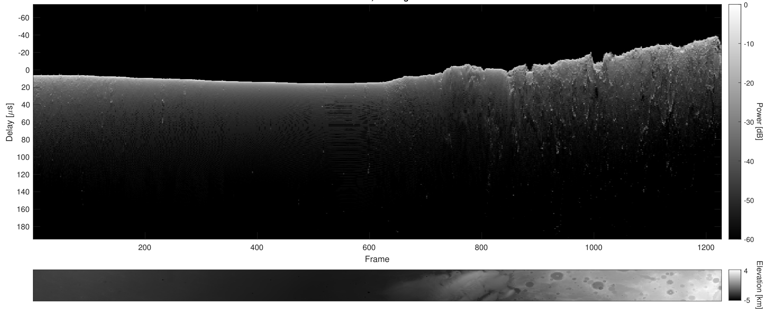
Orbit 5204, Cluttergram
