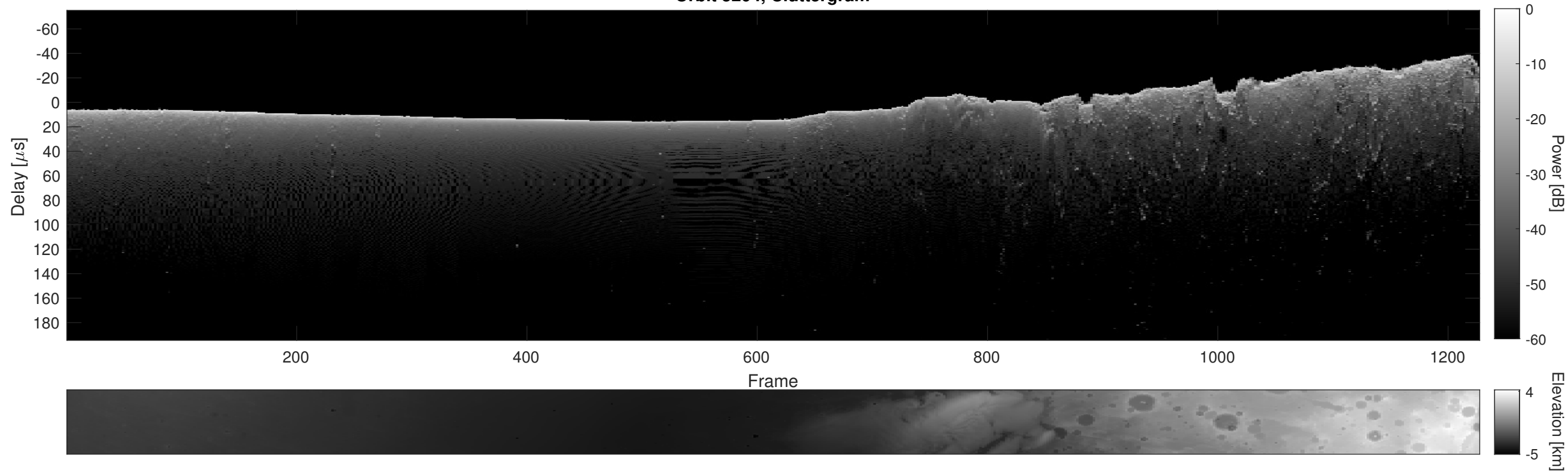
Orbit 5204, Cluttergram
