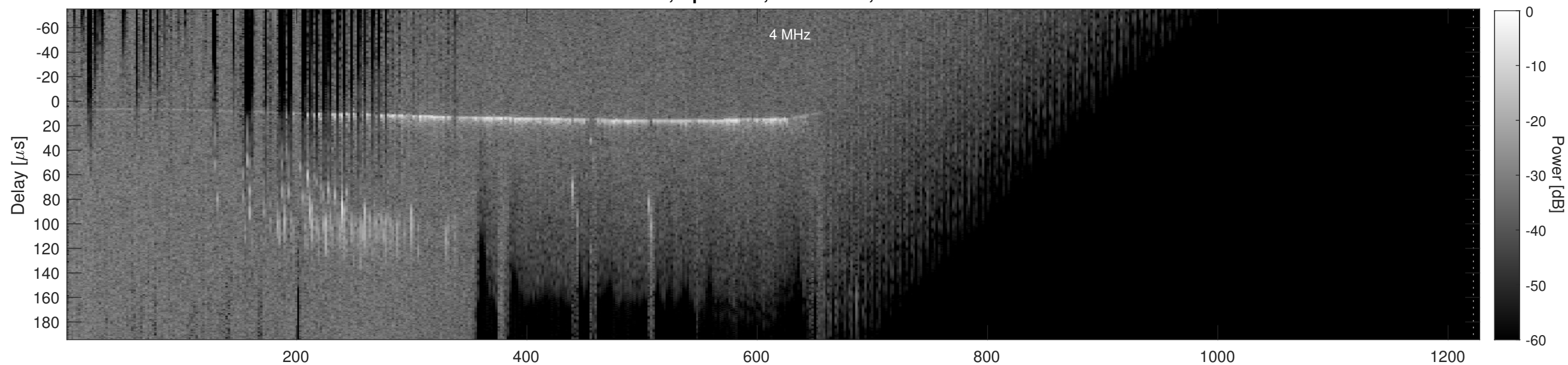
Orbit 5204, Cluttergram
