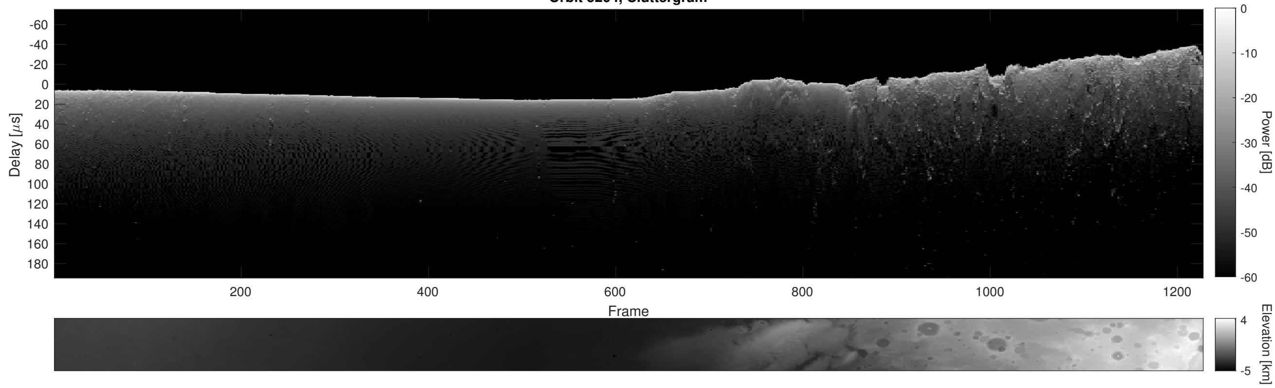
Orbit 5204, Cluttergram
