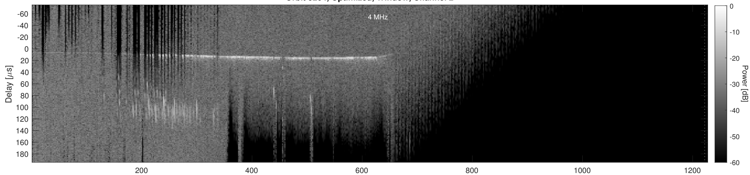
Orbit 5204, Cluttergram
