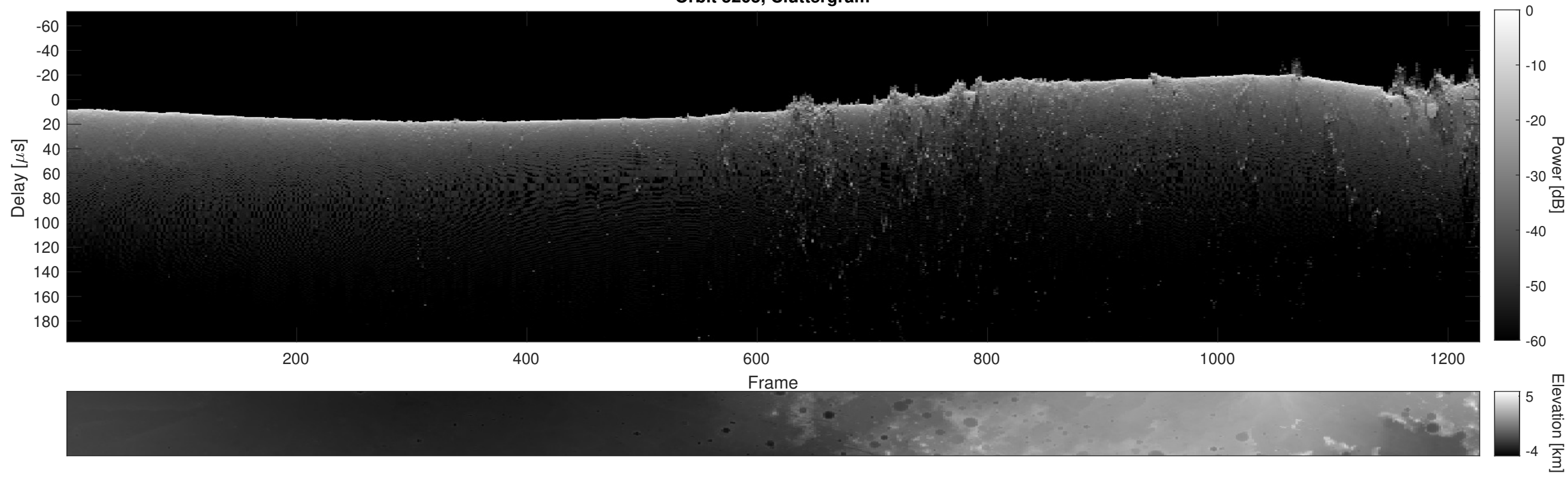
Orbit 5205, Cluttergram
