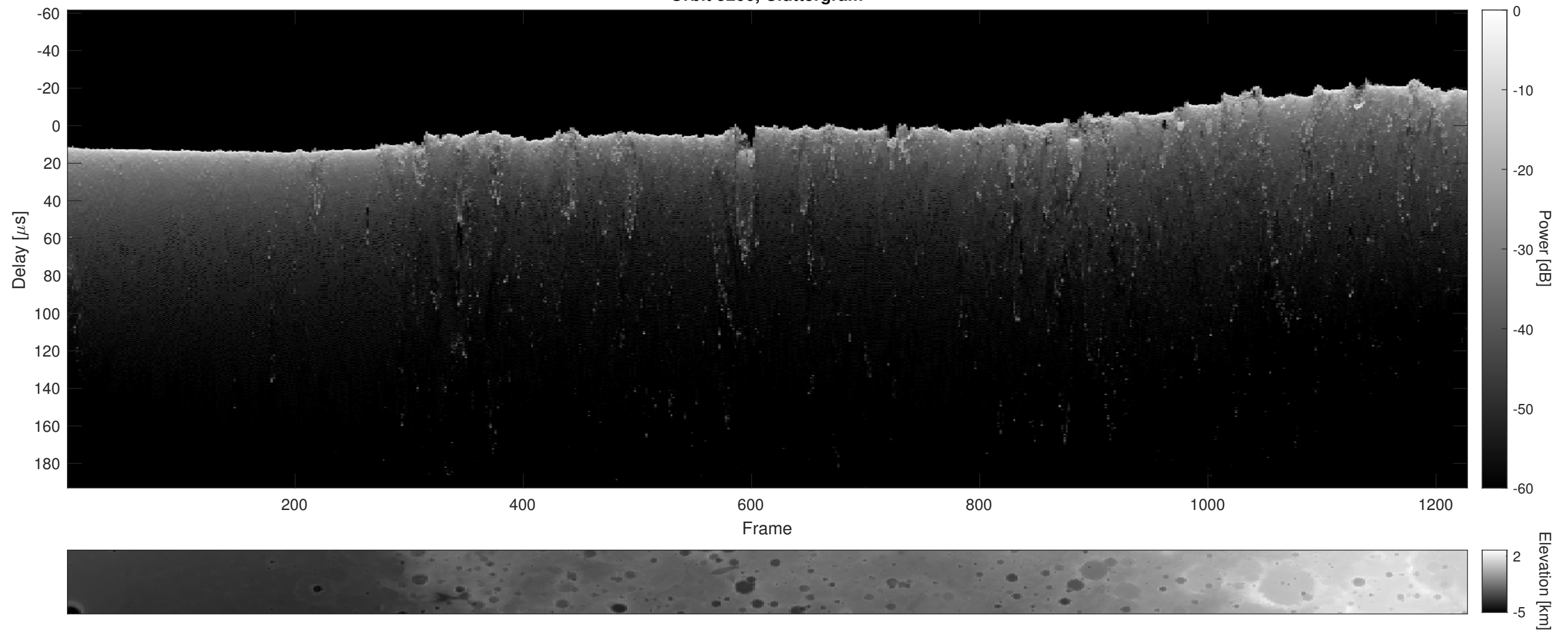
Orbit 5206, Cluttergram
