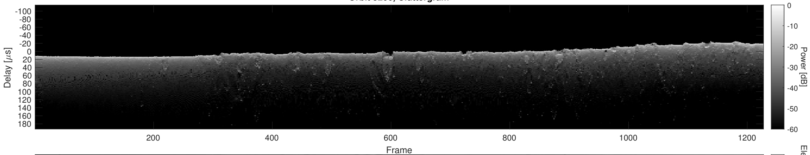
Orbit 5206, Cluttergram
