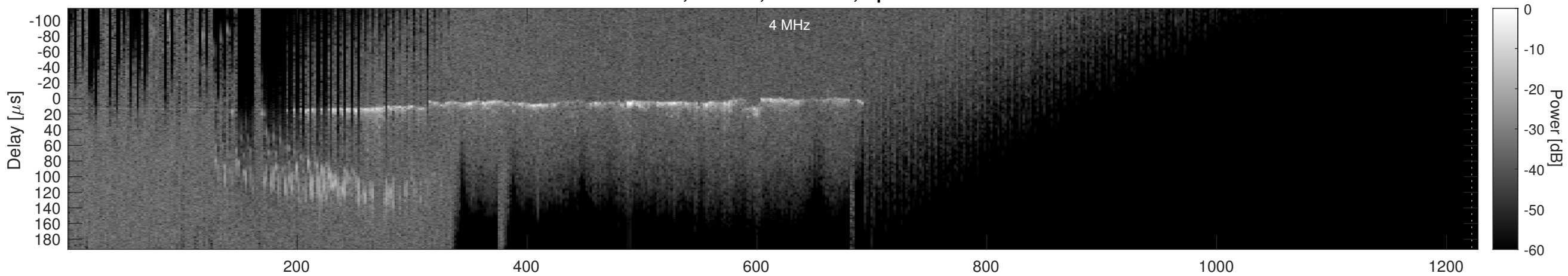
Orbit 5206, Cluttergram
