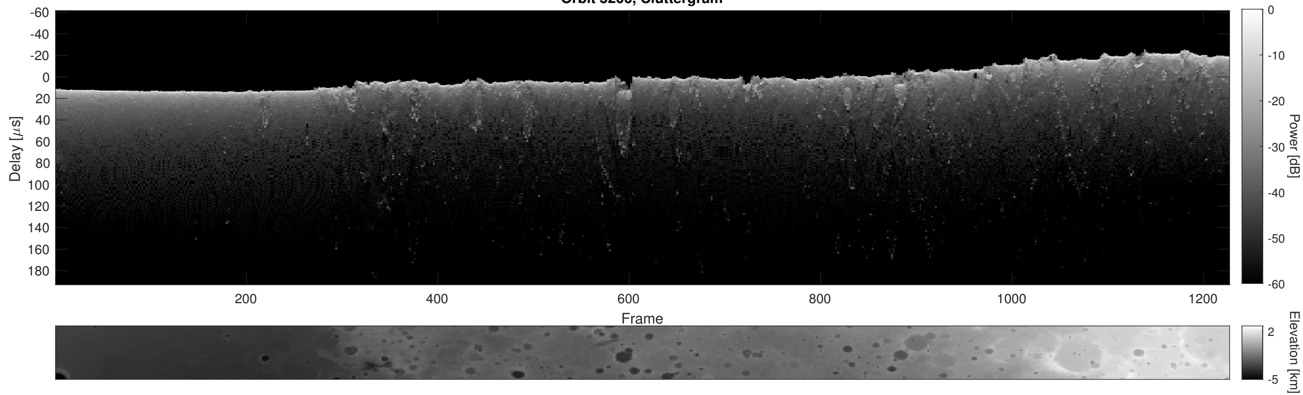
Orbit 5206, Cluttergram
