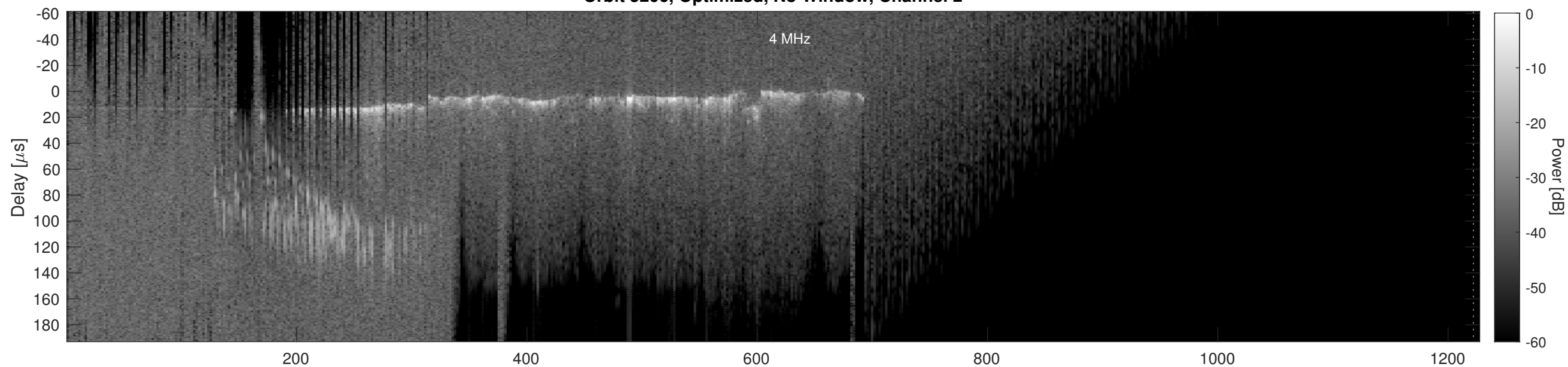
Orbit 5206, Cluttergram
