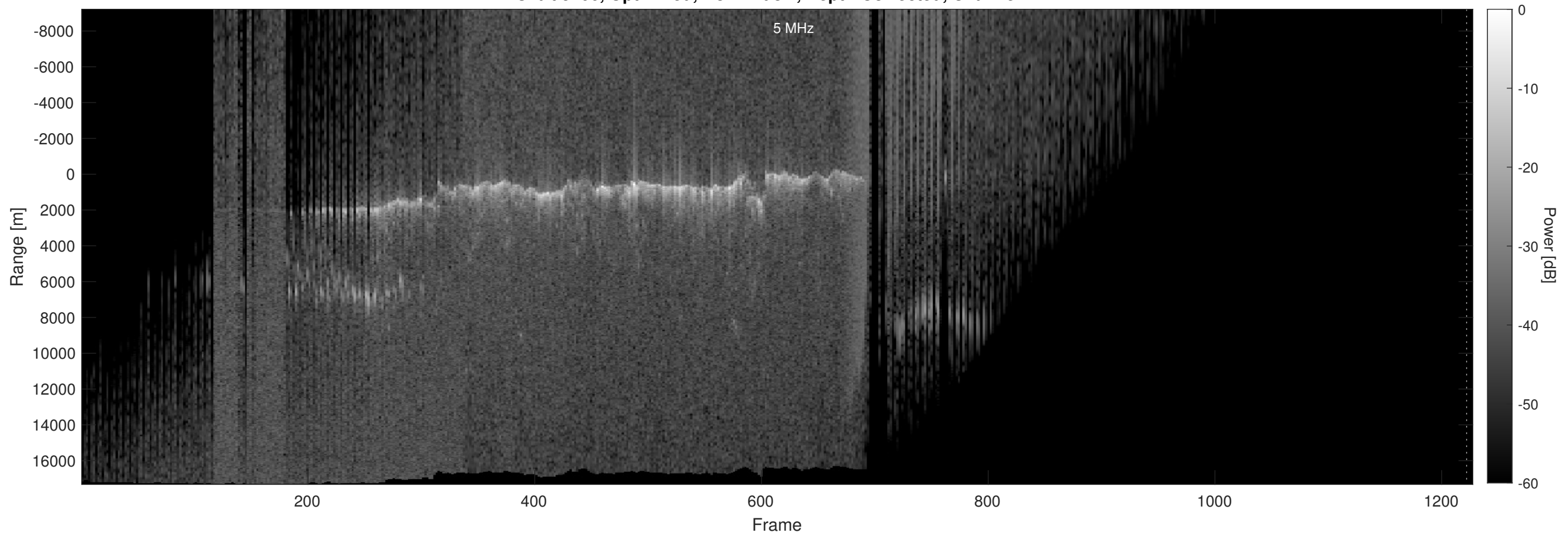
Orbit 5206, Optimized, No Window, Depth-Corrected, Channel 2
