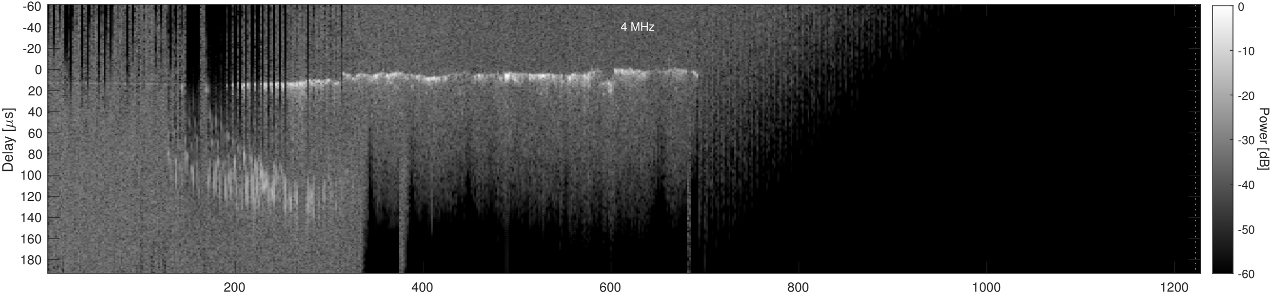
Orbit 5206, Cluttergram
