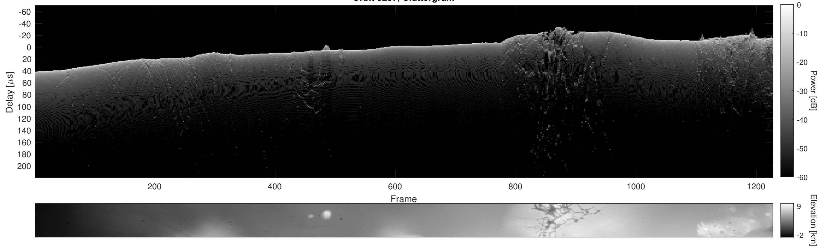
Orbit 5207, Cluttergram
