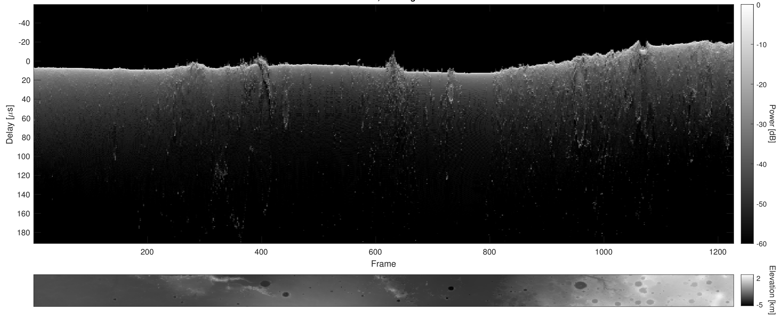
Orbit 5208, Cluttergram
