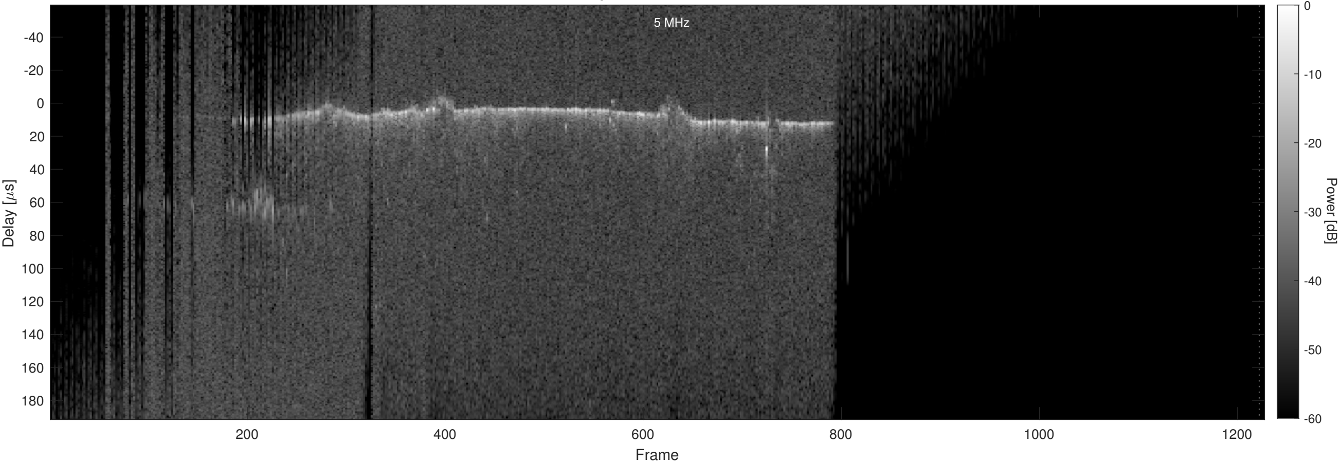
Orbit 5208, Optimized, Window, Channel 2
