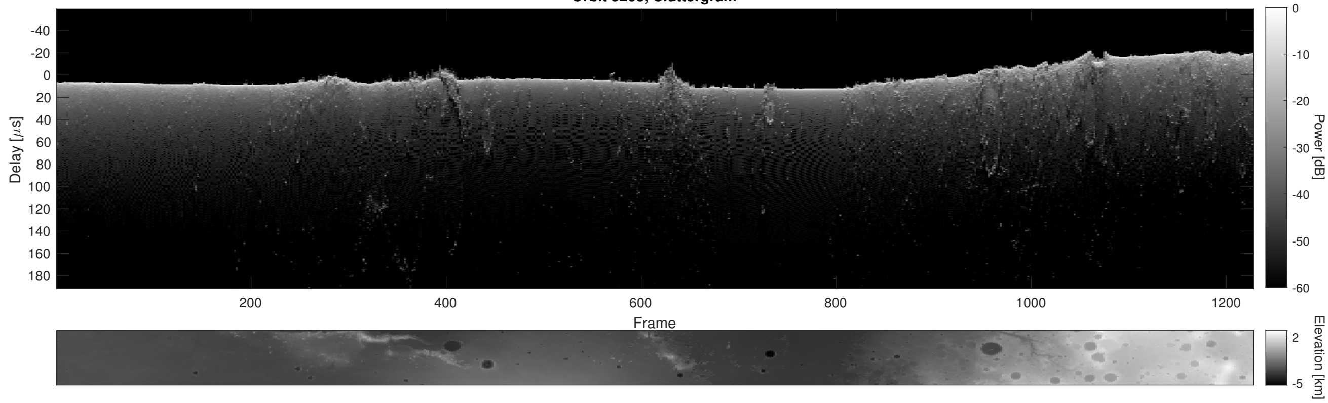
Orbit 5208, Cluttergram
