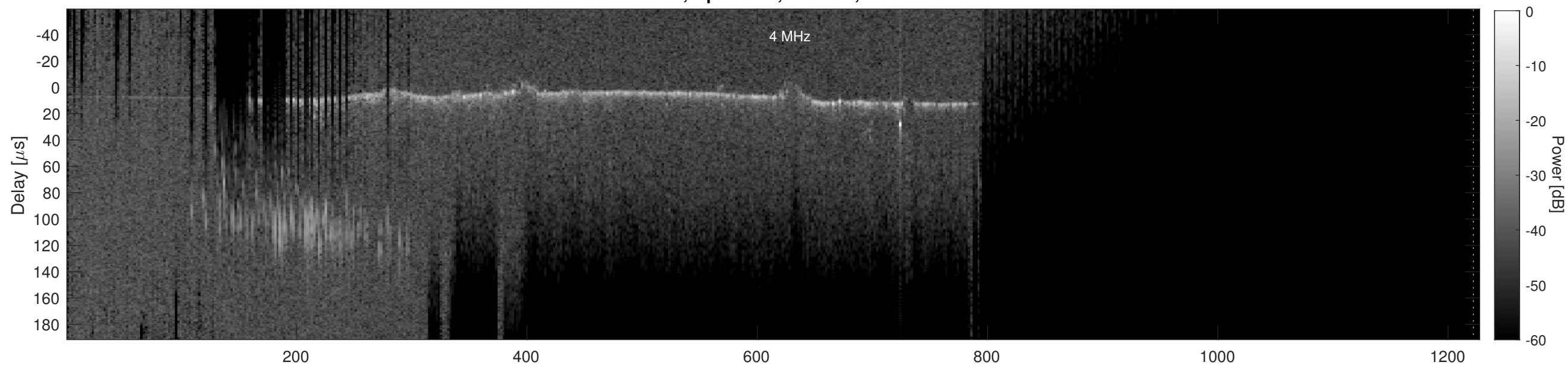
Orbit 5208, Cluttergram
