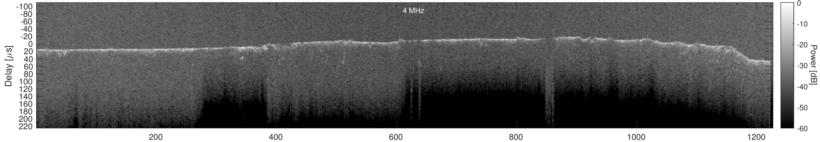
Orbit 5209, Cluttergram
