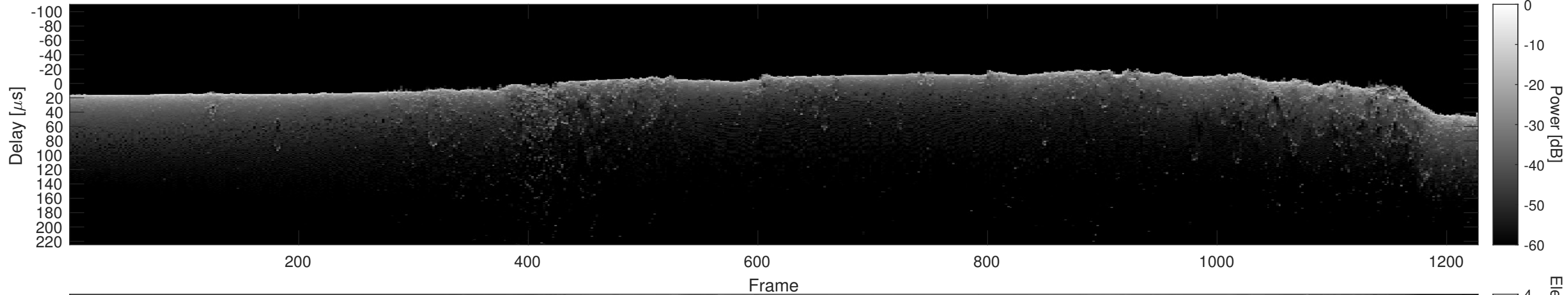
Orbit 5209, Cluttergram
