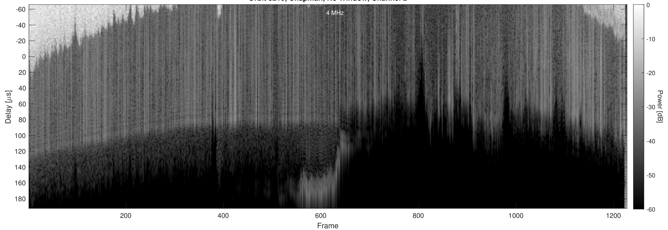
Orbit 5210, Chapman, No Window, Channel 2
