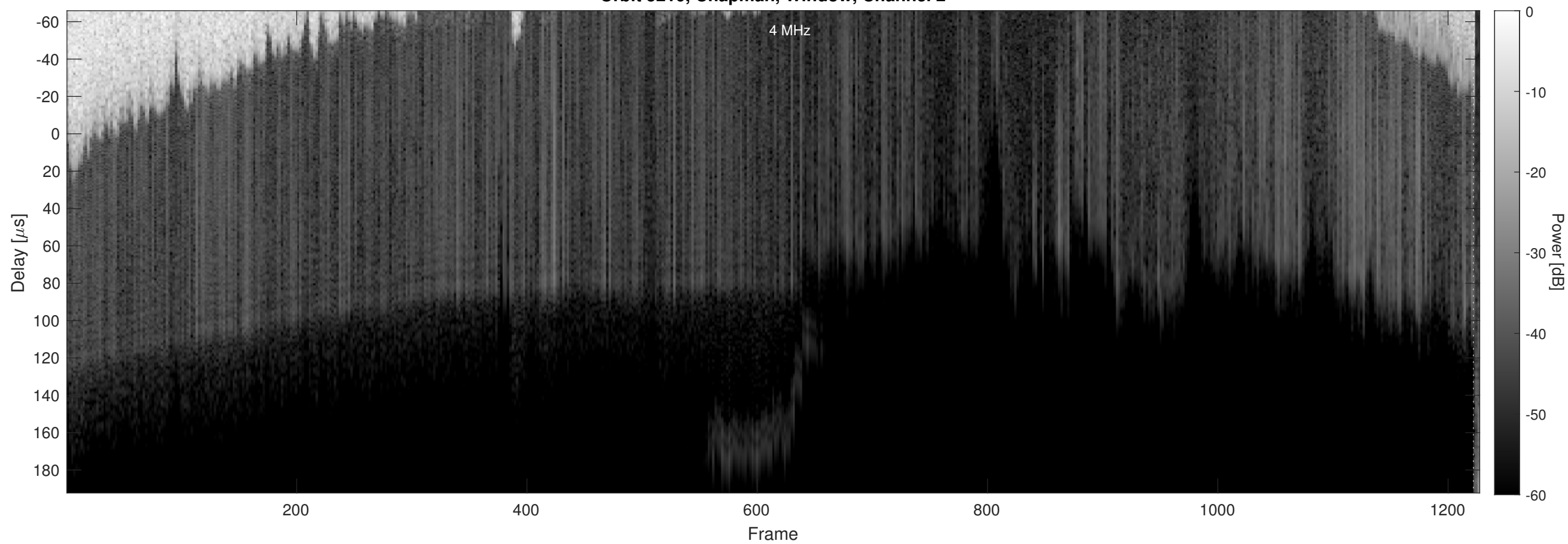
Orbit 5210, Chapman, Window, Channel 2
