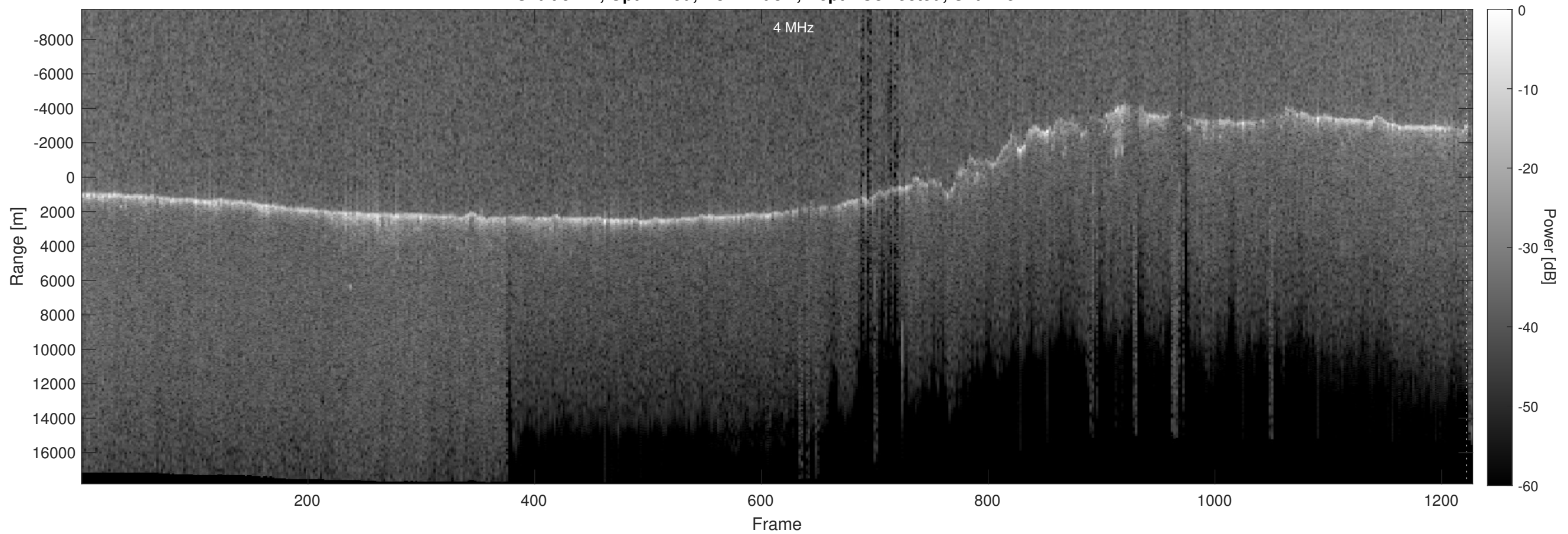
Orbit 5212, Optimized, No Window, Depth-Corrected, Channel 2
